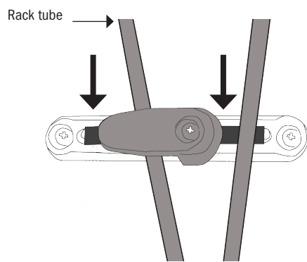
Mounting in Quick-Lock1 system
