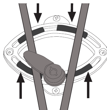
Mounting in Quick-Lock2 system
